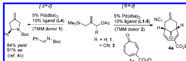
Figure 1. Phosphoramidite ligand screen. Reactions performed at 0.1 M in toluene with 5 mol % Pd(dba) 2 , 10 mol % ligand, 1.0 equiv 3a , 1.6 equiv 2 , 0–4 °C for 15 h; ee determined by chiral HPLC.
