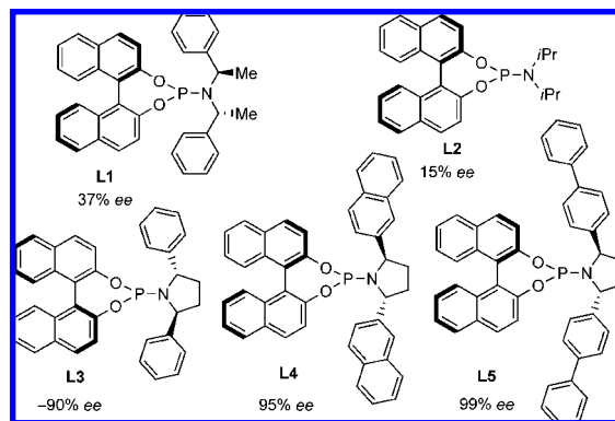
Figure 1. Phosphoramidite ligand screen. Reactions performed at 0.1 M in toluene with 5 mol % Pd(dba) 2 , 10 mol % ligand, 1.0 equiv 3a , 1.6 equiv 2 , 0–4 °C for 15 h; ee determined by chiral HPLC.
